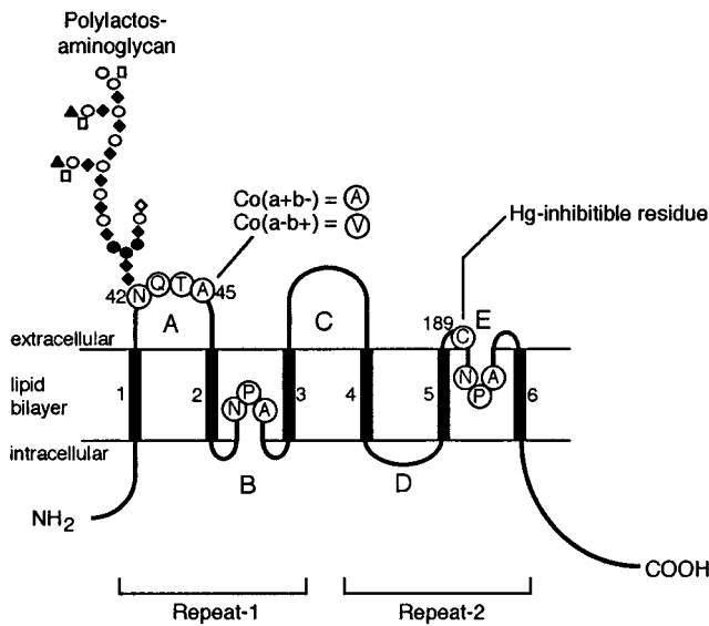
FIGURE 1 Schematic diagram representing the structure of a monomeric subunit of the AQP1 water transport protein.
